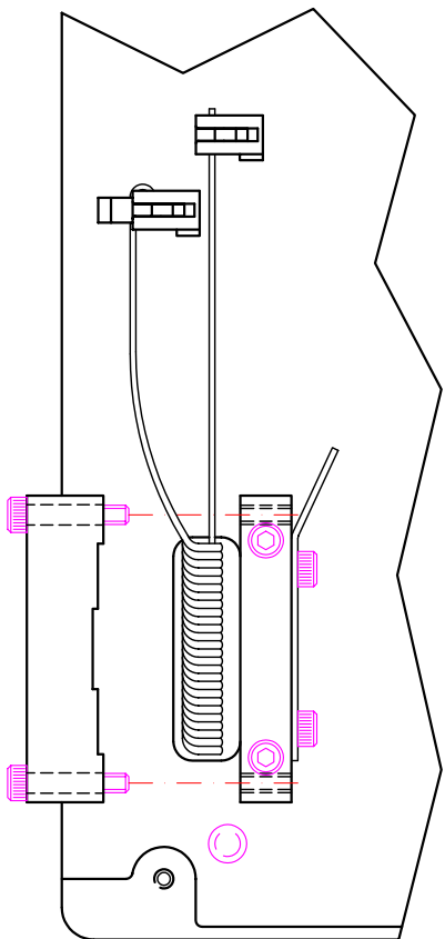
Part View of 53CL Printer Body (Cassette Removed)
